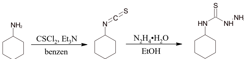
Figure 3. Synthesis scheme of N -cyclohexylhydrazinecarbothioamide from amine
