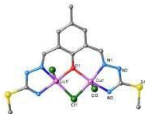
Figure 5. X-ray molecular structure of 2. Unit cell Parameters: a=9.002 , b=23.117 , c=14.882 , \alpha=90 , \beta=105.48 , \gamma=90 ; Sp. Gr. I2/a .
