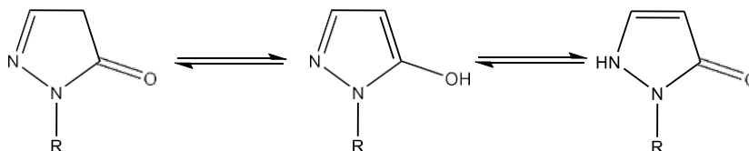
Figura 2. Tautomeria pirazolonelor
