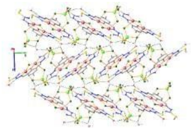
Figure 3. Partial view of the crystal structure packing along a crystallographic axis of 4 showing the formation of 2D supramolecular layer. H-bonds are drawn as dashed-black lines.
