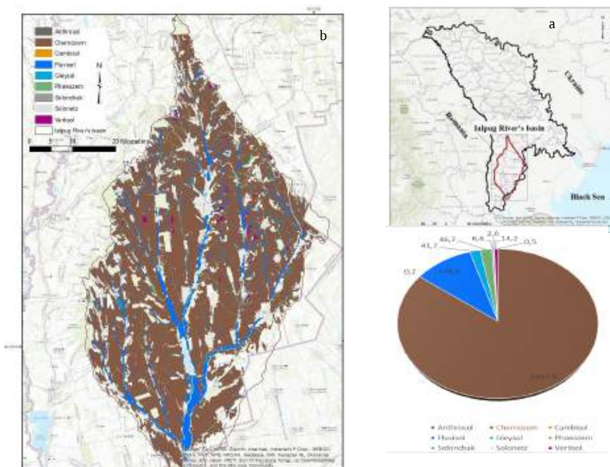
Fig. 2. Study area delimitation (a); Pedological map of Ialpuș River's basin (b); Soil types' areas distribution within the basin, km 2 .
