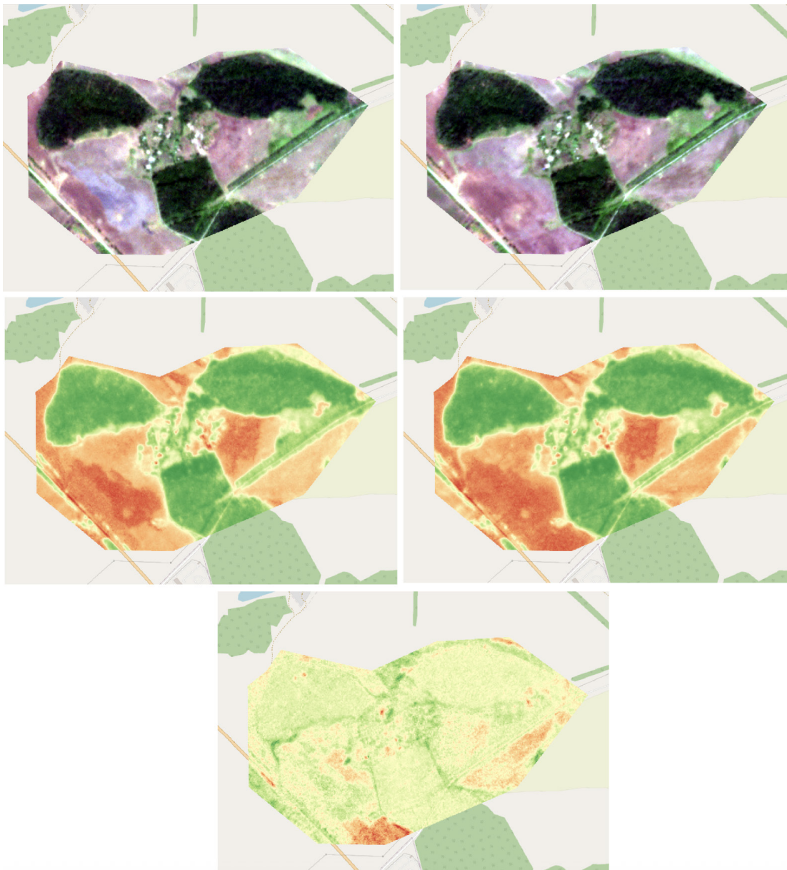
Fig. 7. Layer showing changes in vegetation cover over 10 days in an area of intense combat operations
