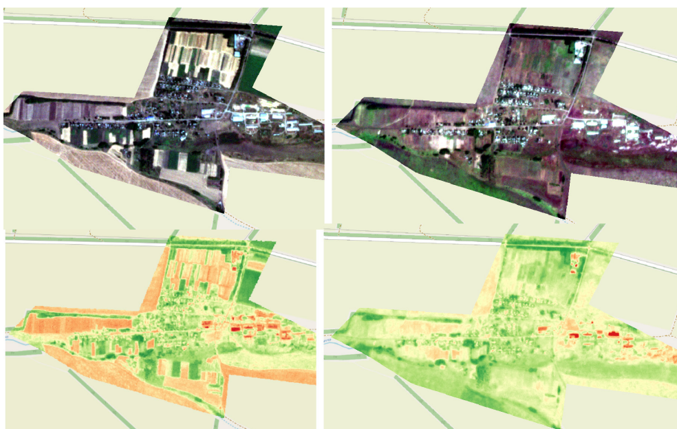
Fig. 6. Comparison of satellite images of the village of Velykyi Vyselok in August 2021 and August 2025
