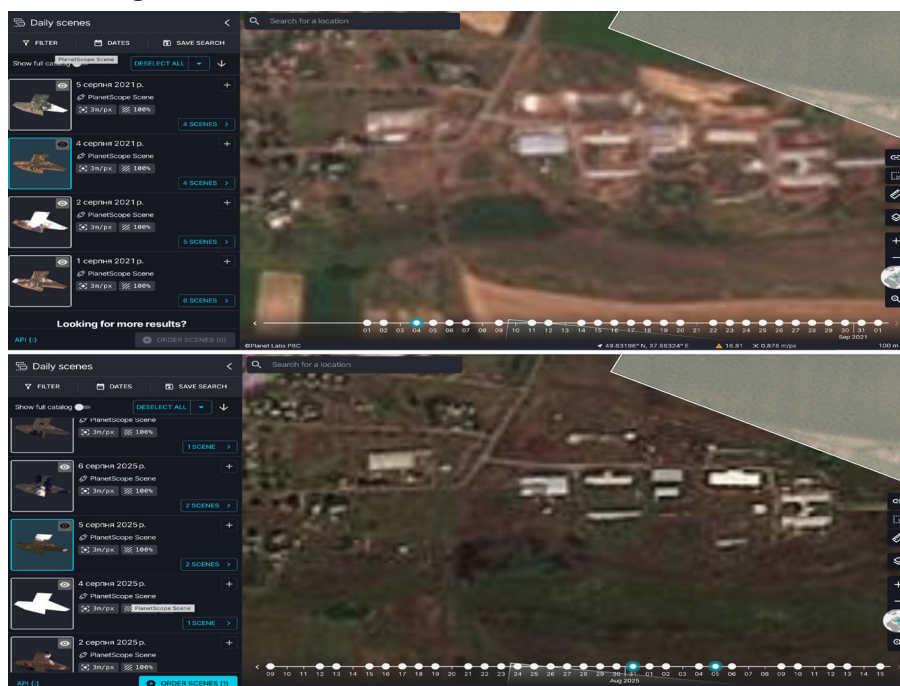
Fig. 3. Comparison of photographs
