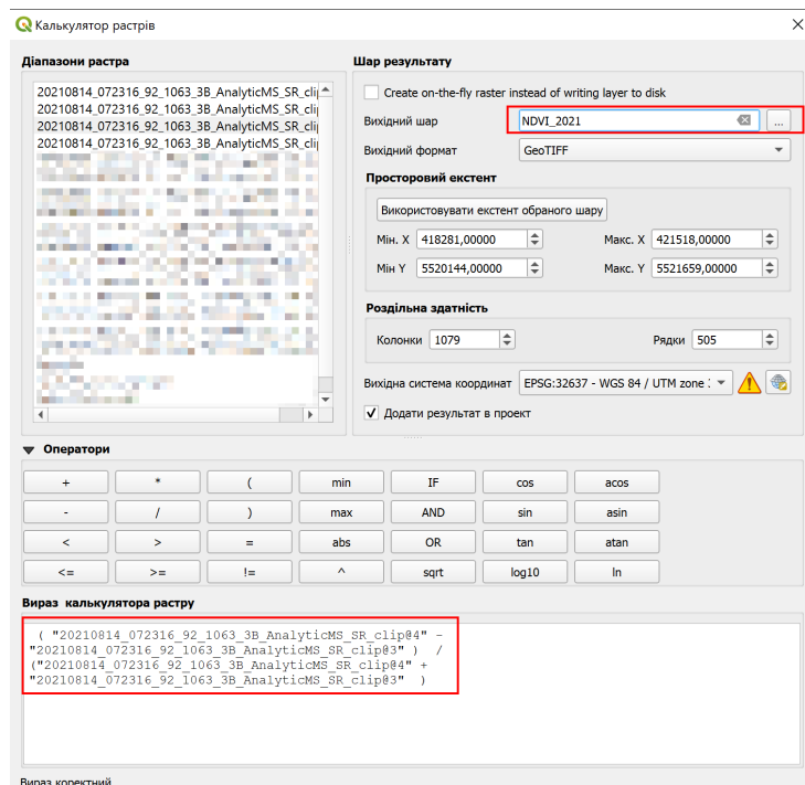
Fig. 5. Raster calculator
