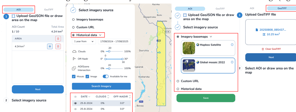
Fig. 1. Determining the data source for analysis
